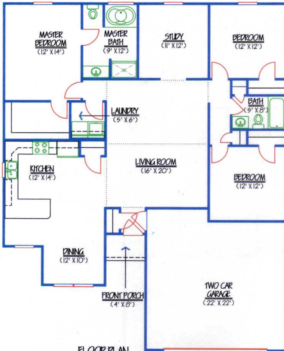
FLOOR PLAN
