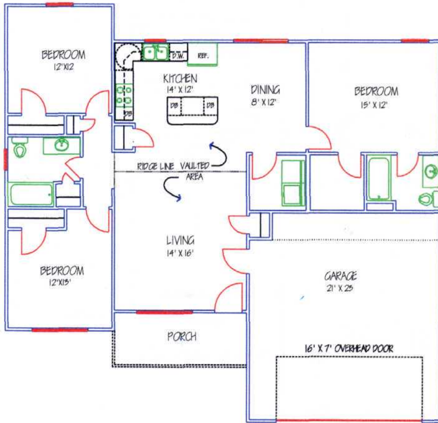
FLOOR PLAN
