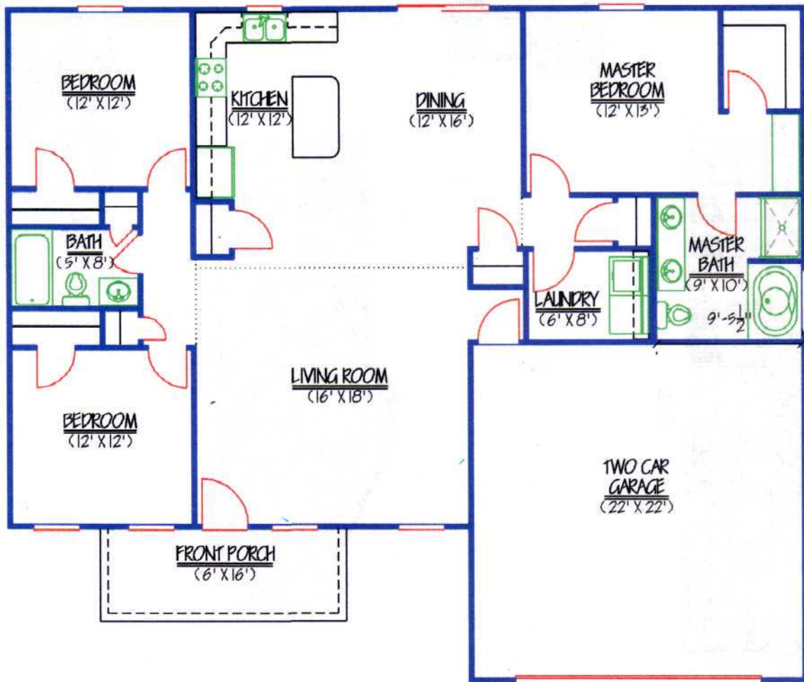
FLOOR PLAN
