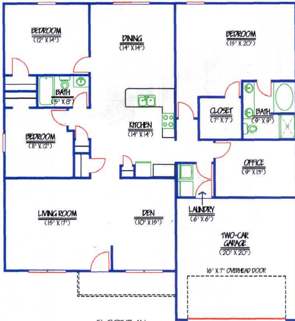
FLOOR PLAN
