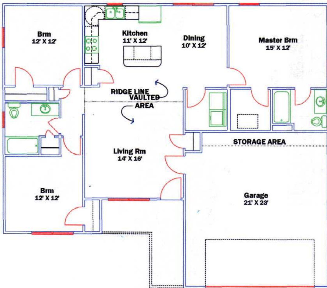
FLOOR PLAN
