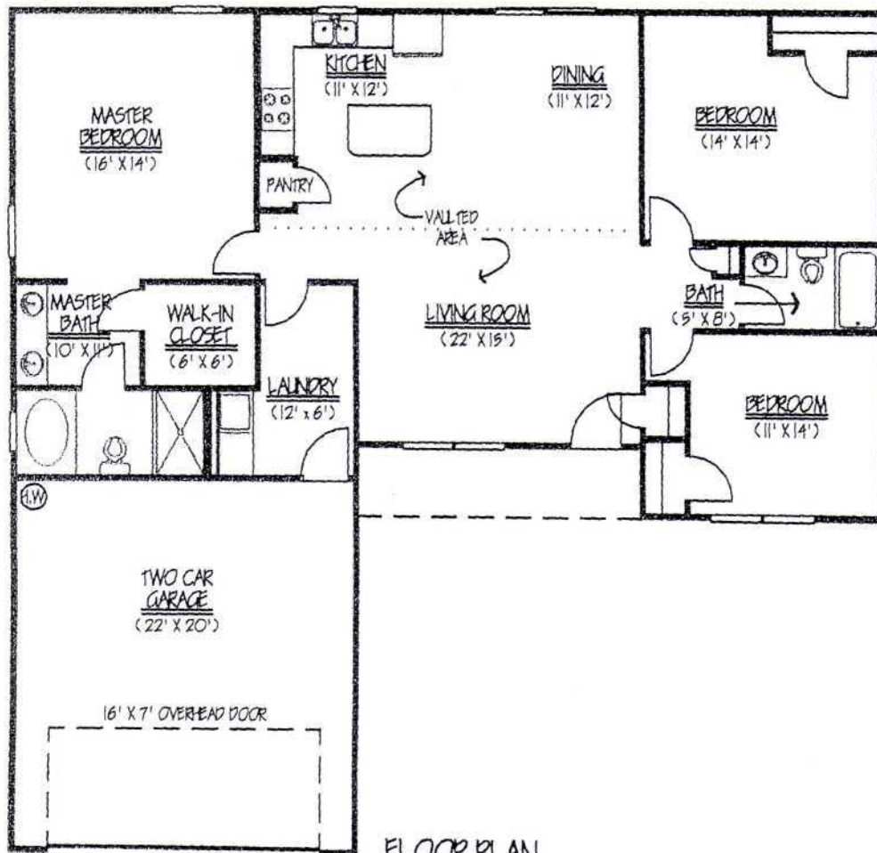
FLOOR PLAN
